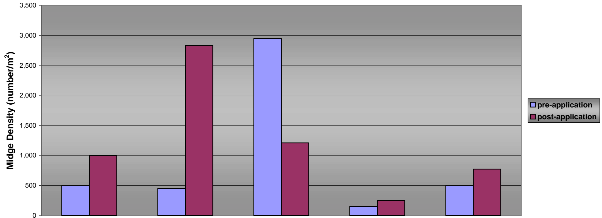
Figure 5. Straits Pond Deepwater Pre-Application Midge Abundance vs Mean Post Application Midge Abundance (2003)
